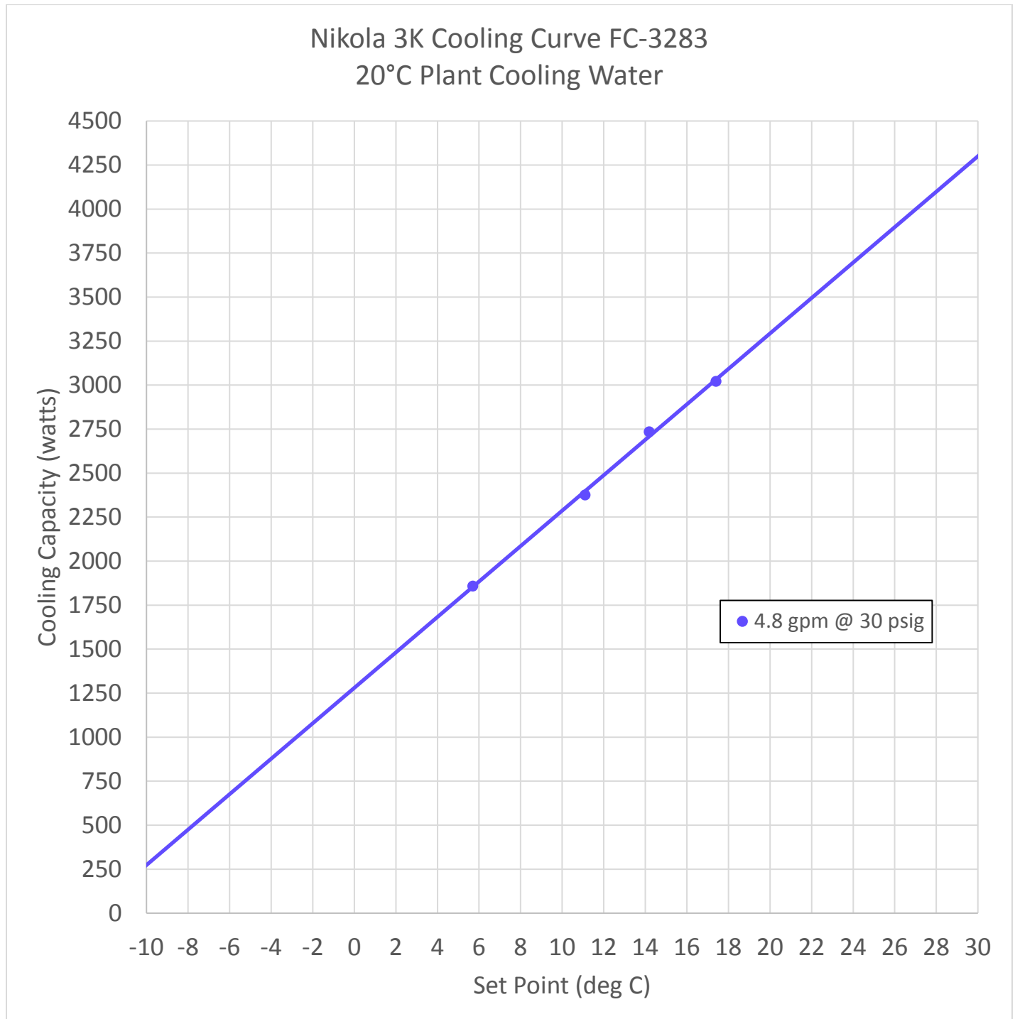
Figure 1C: Nikola 3K Cooling Capacity with Fluorinert or Galden Fluids
