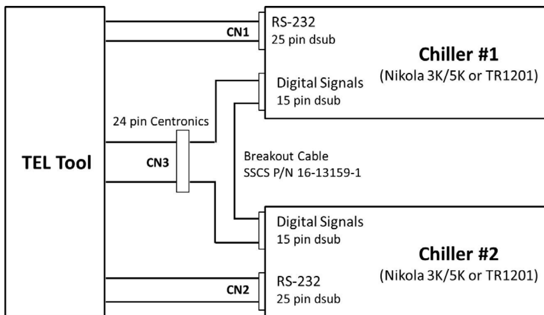
Figure 7: TEL Unity II or Unity M Signal Hook-up
