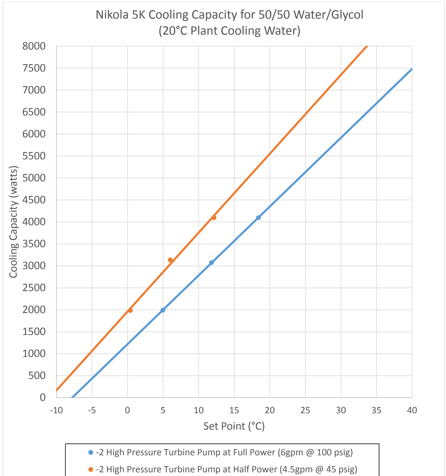
Figure 1A: Nikola 5K Cooling Capacity with 50/50 Water/Ethylene Glycol
