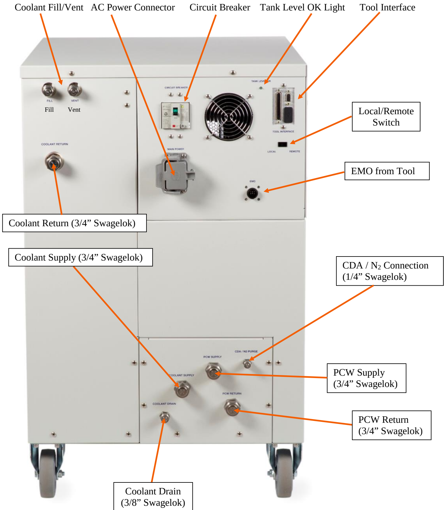
Figure 3: Rear View
