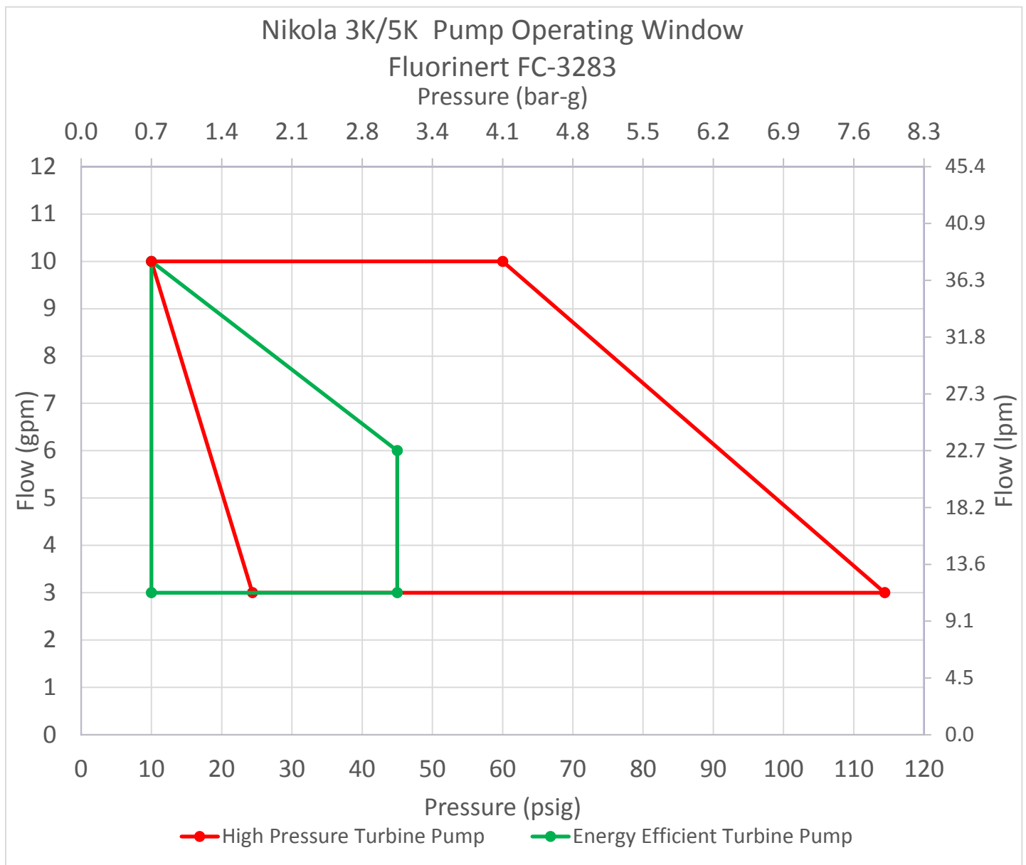
Figure 2B: Nikola 3K/5K Pump Operating Window 50/50 Water/Ethylene Glycol
