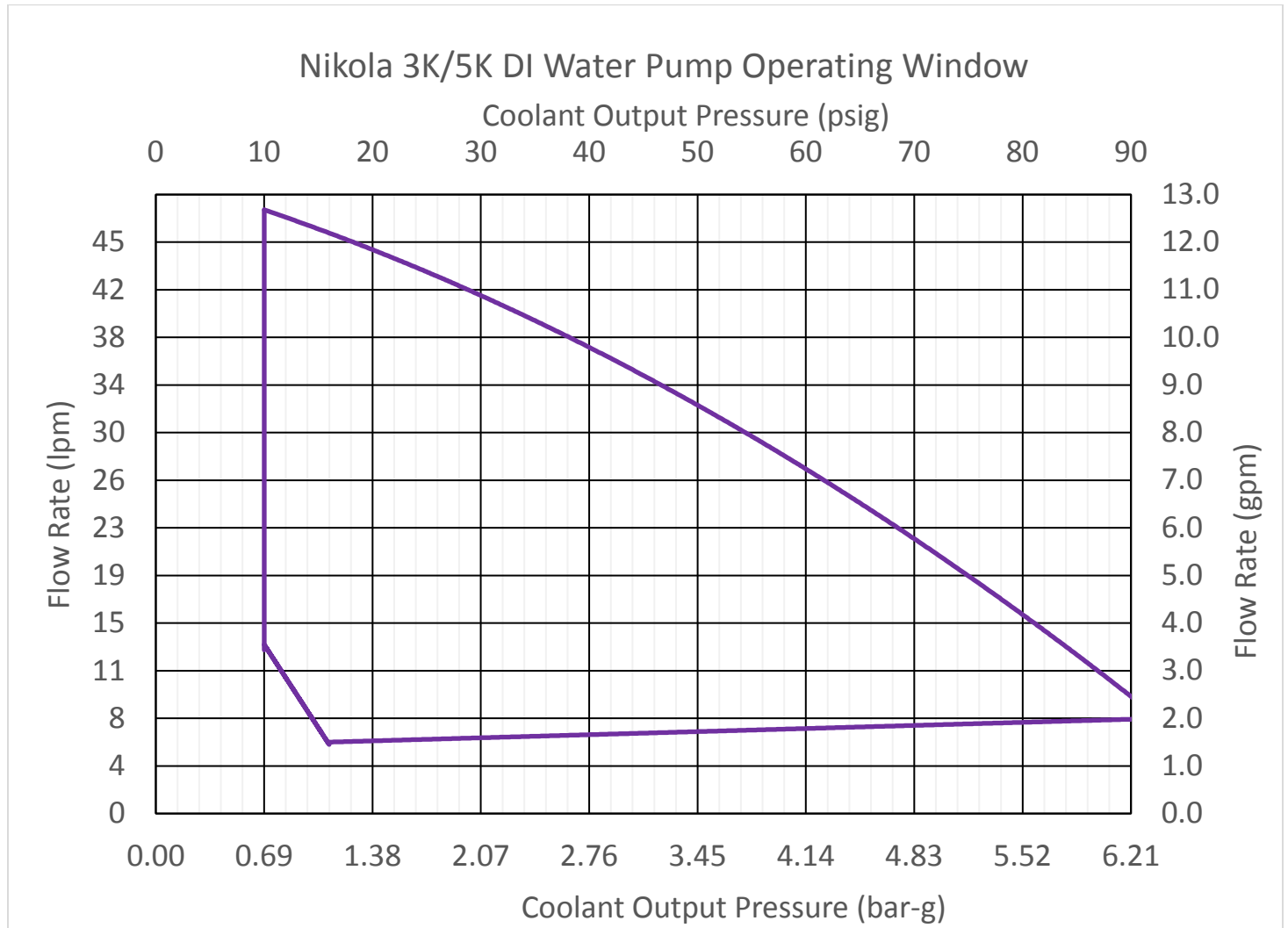
Figure 2C: Nikola 3K/5K Special 100% DI Water Pump 1 Operating Window
