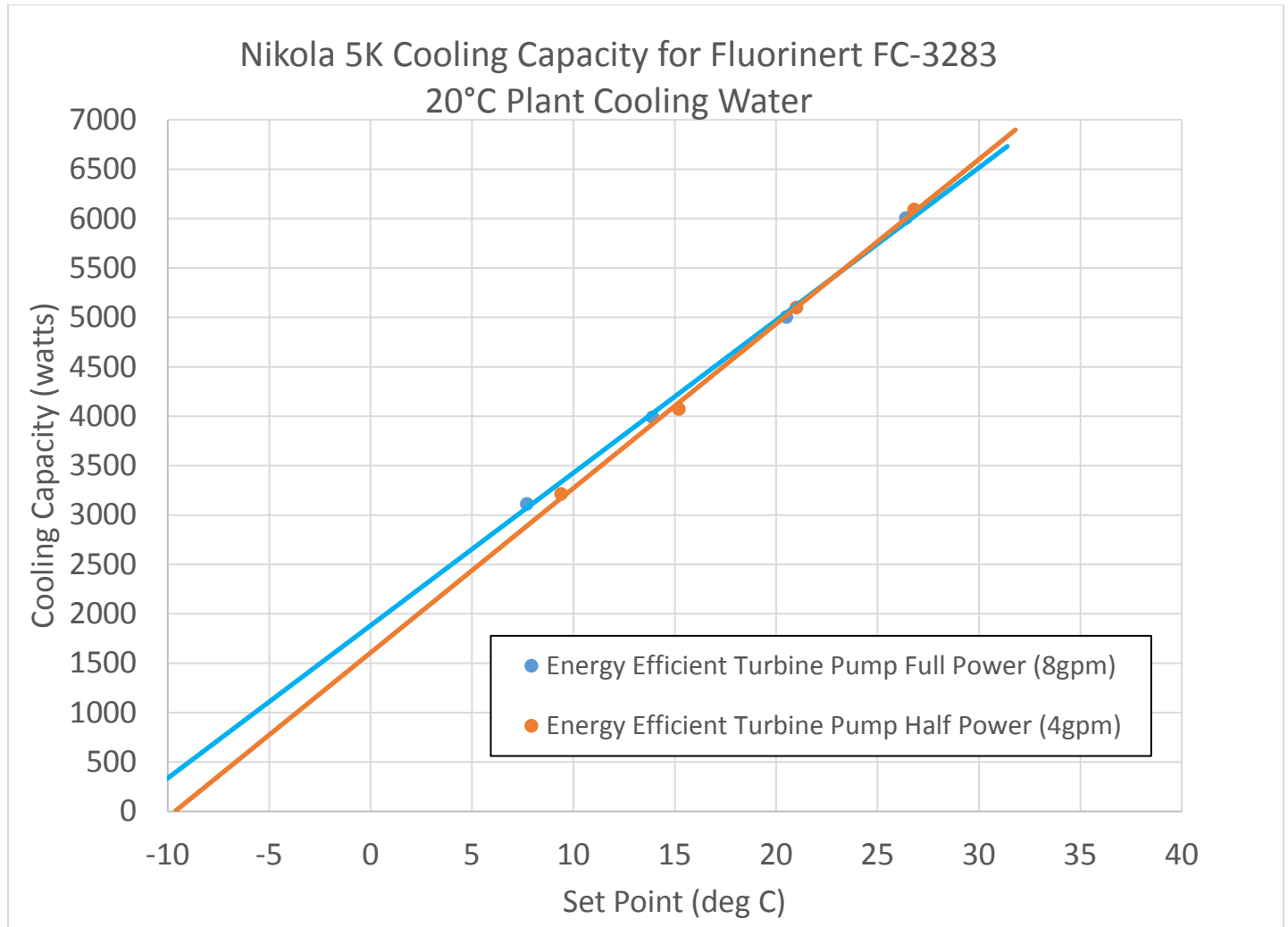
Figure 1B: Nikola 5K Cooling Capacity with Fluorinert or Galden Fluids
