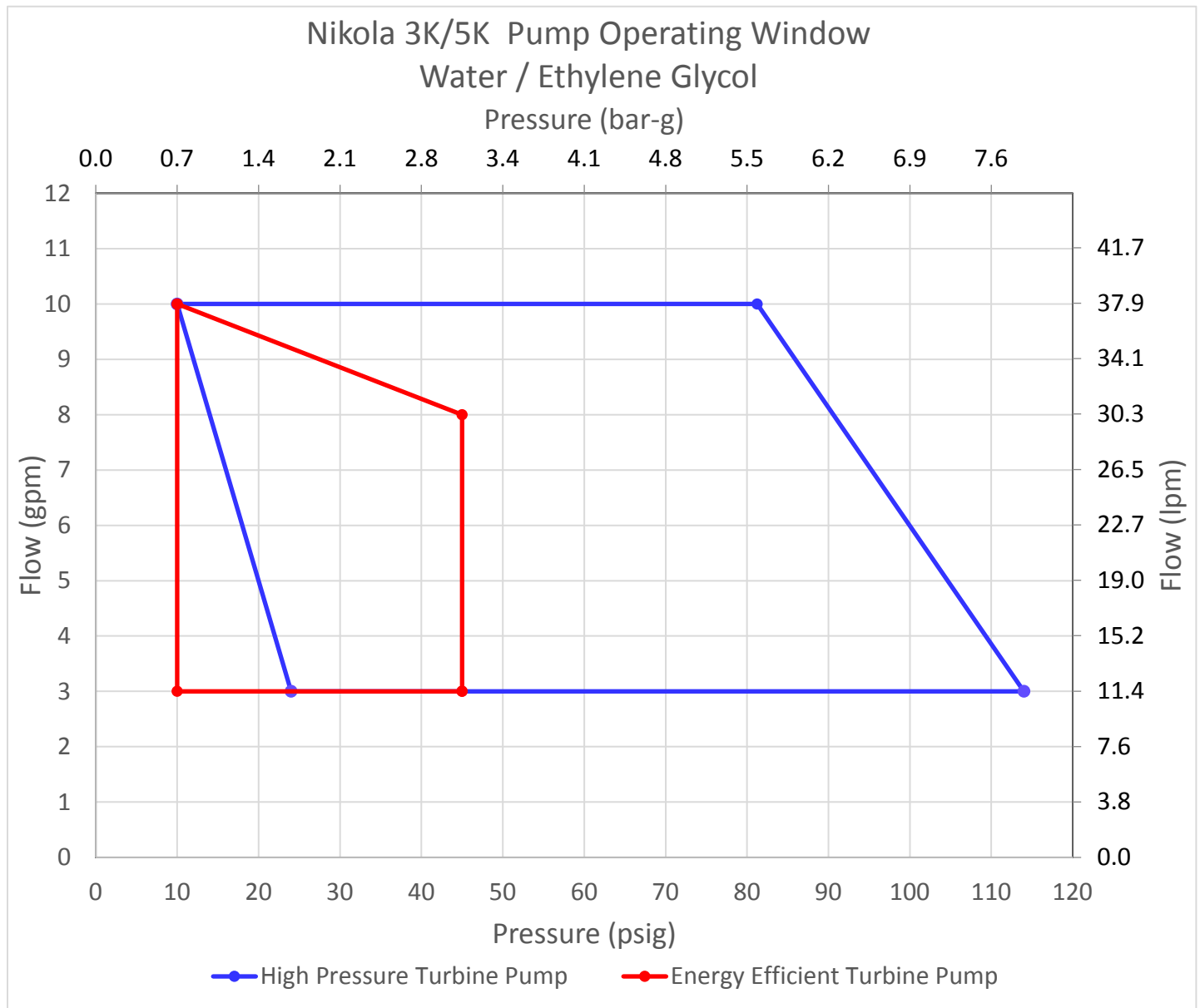
Figure 2A: Nikola 3K/5K Pump Operating Window - 50/50 Water/Ethylene Glycol
