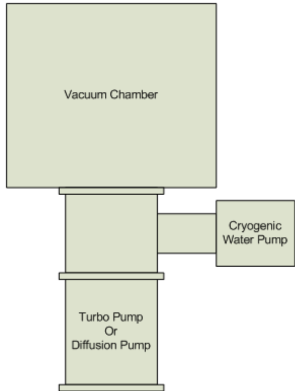
Figure 2 – Cryogenic Water Pump In-Line with Turbo/Diffusion Pump
