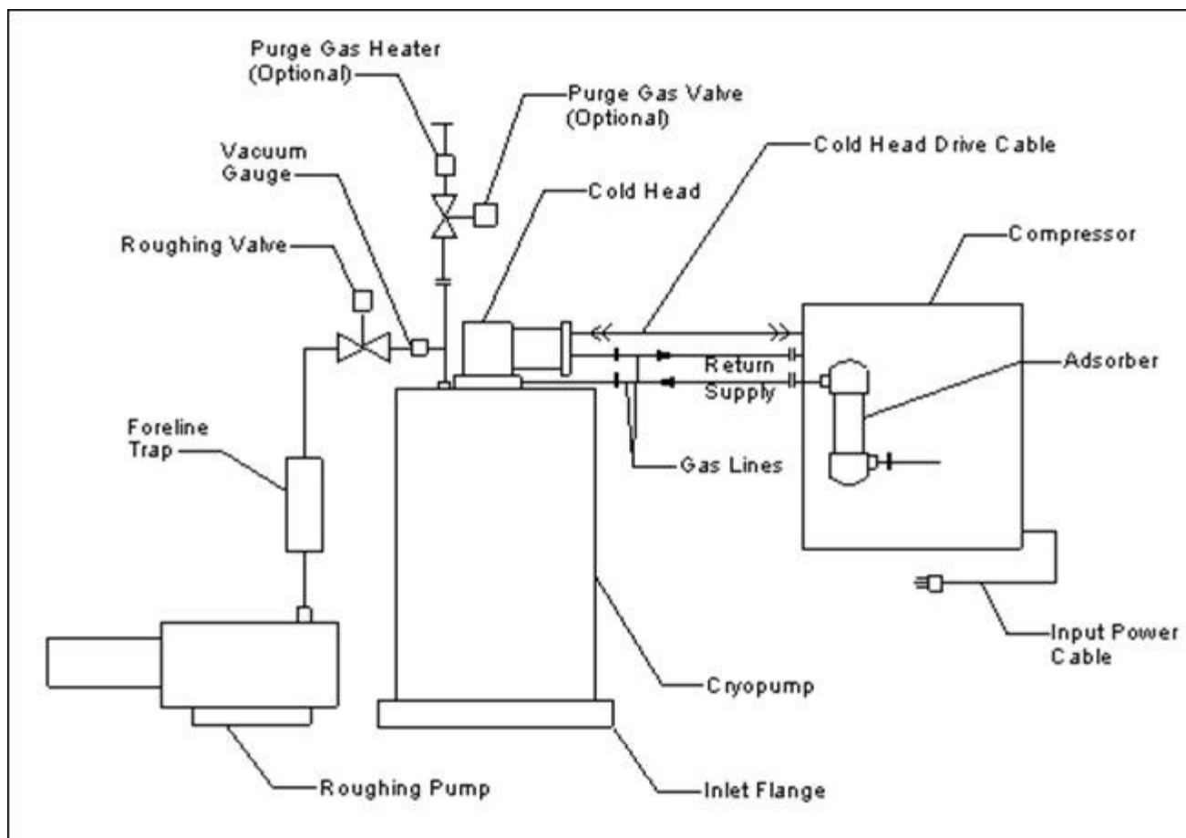
Figure 10 – Connection Diagram
