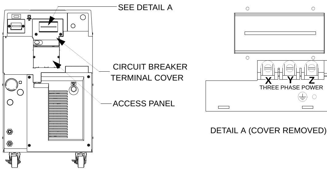
Figure 4-2: 9700A Compressor Circuit Breaker Terminals
