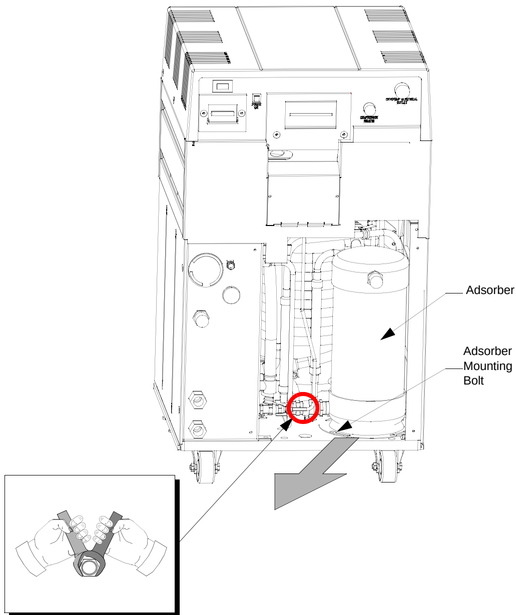
Figure 6-2: Adsorber Location in the 9700A Compressor (Rear Panel Removed)
