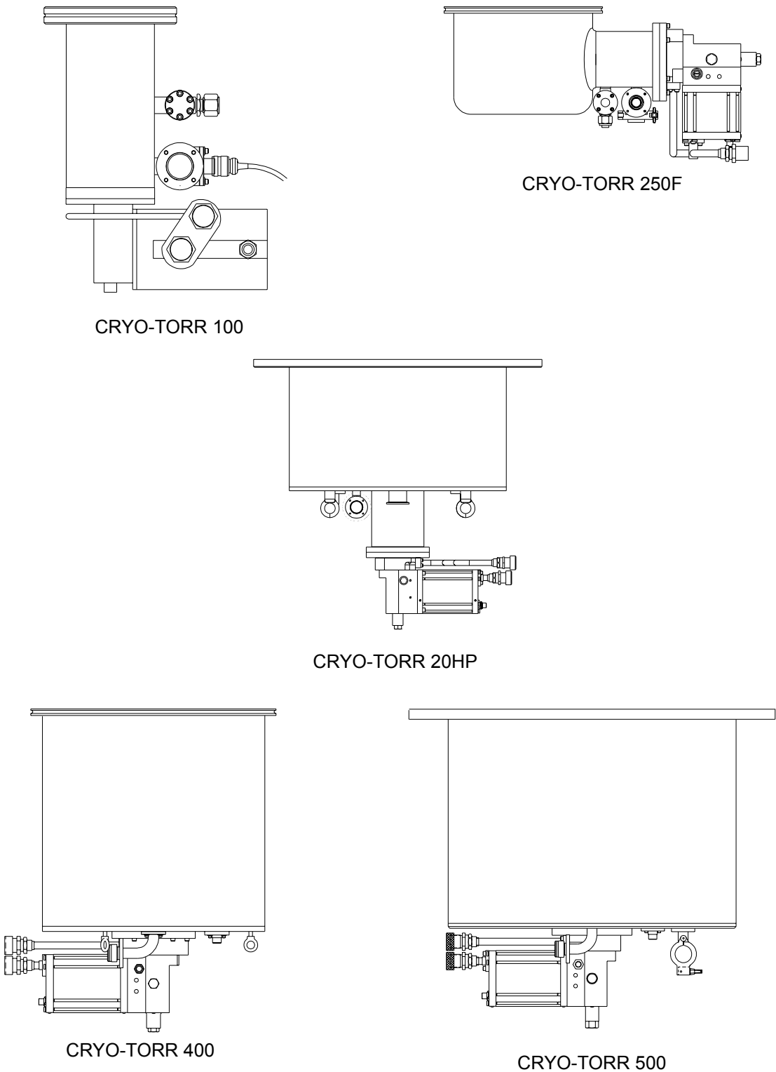
Figure 1-2: Cryo-Torr Pumps
