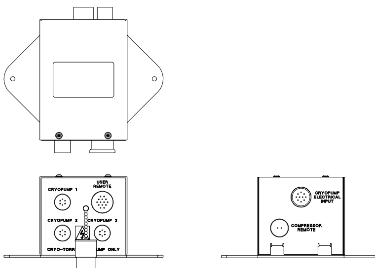
Figure 1-4: Cryo-Torr Interface
