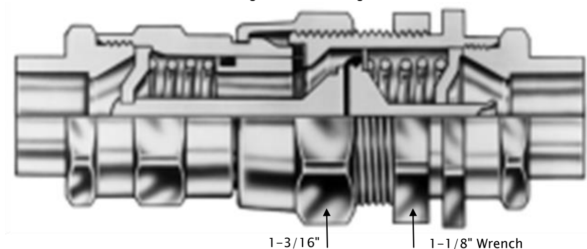
Figure 18 – Self sealing Connector
