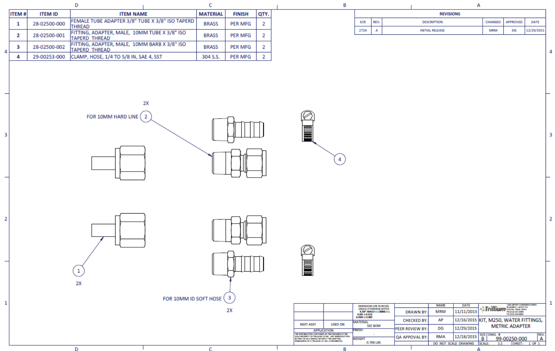
Figure 26 – 99-00250-000 Kit Contents
