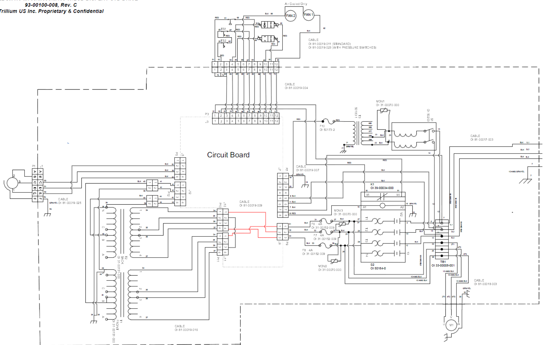
Figure 16 – M700 Water High Volt Standard Drive Schematic
