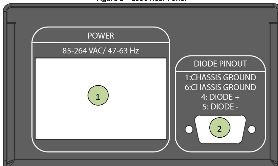
Figure 1 – E350 Rear Panel
