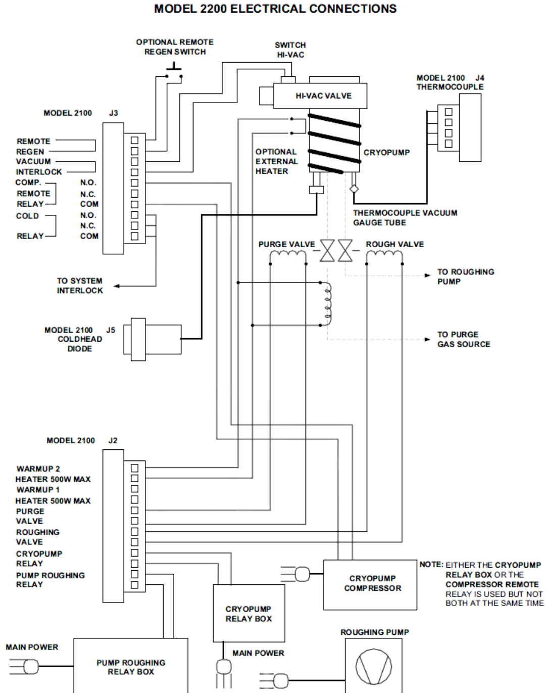
Figure 1 – Model 2200/2200E Electrical Connections Schematic
